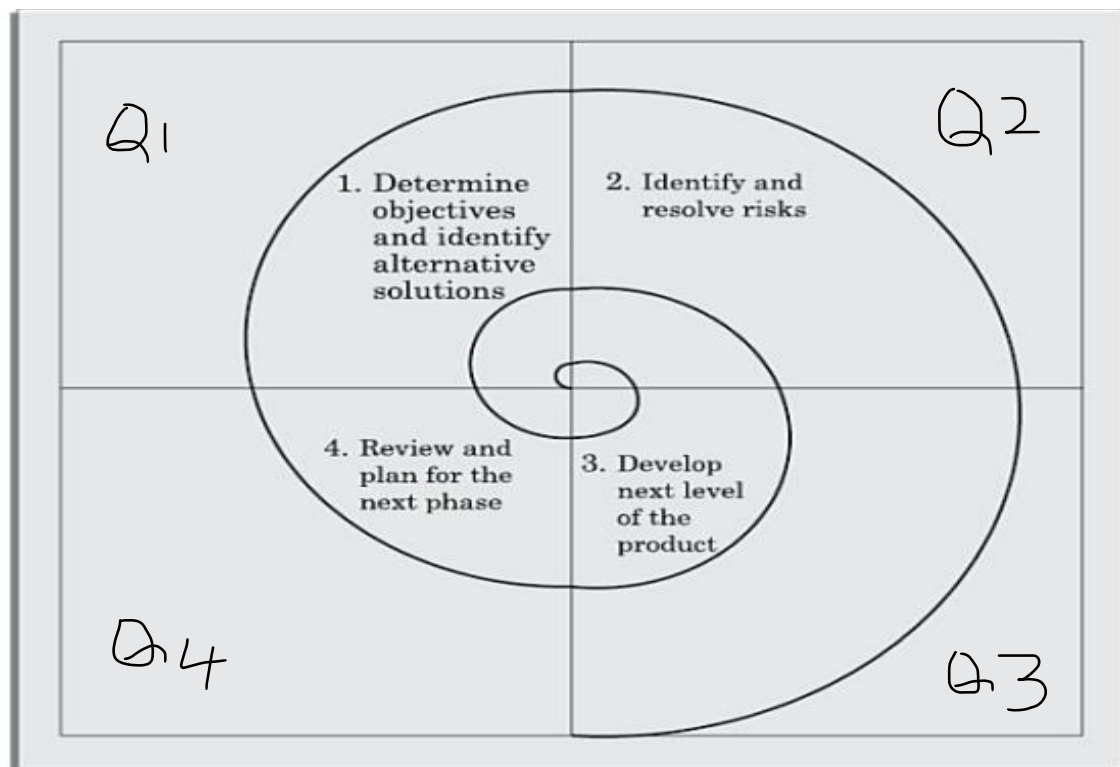
Figure 2.10: Spiral model of software development.
