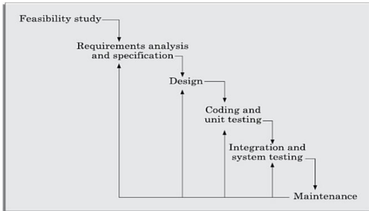
Figure 2.3: Iterative waterfall model.
