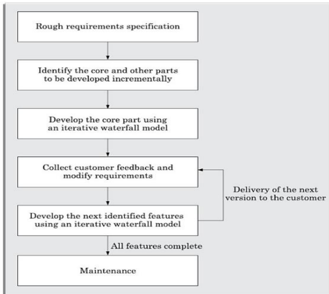
Figure 2.9: Evolutionary model of software development.
