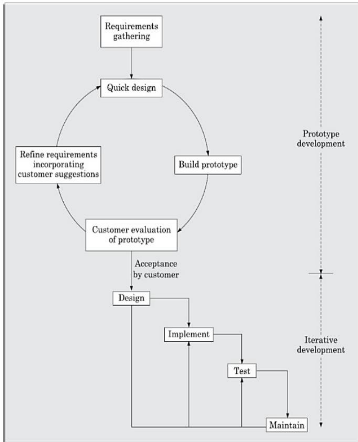
Figure 2.6: Prototyping model of software development.
